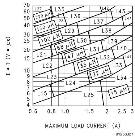
FIGURE7.LM2596-ADJ
