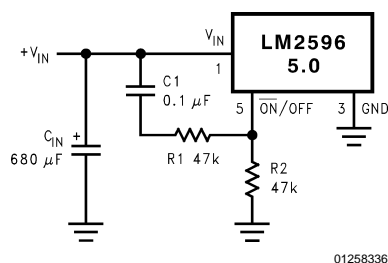
FIGURE 21. Delayed Startup
